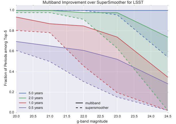
FIG. 9.— Fraction of periods correctly determined for LSST RR Lyrae as a function of the length of the observing season and the mean g -band magnitude, for the multiband periodogram approach (method of this work; solid lines) and single-band supersmoother approach (method of Oluseyi et al. 2012, dashed lines). The multiband method is superior to the single-band supersmoother approach in all cases, and especially for the faintest objects.
