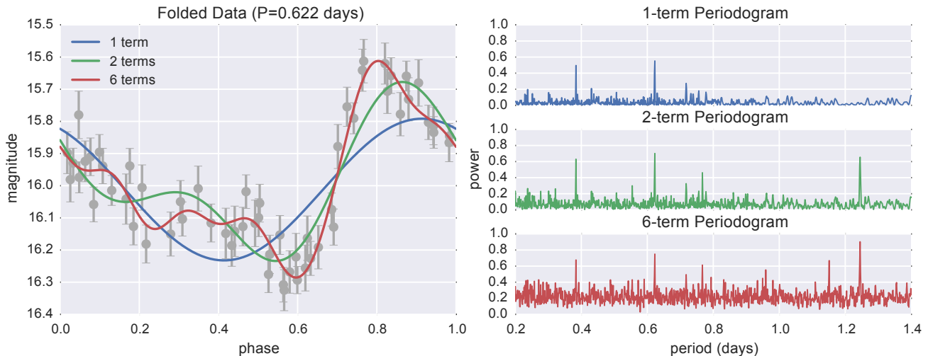
FIG. 3.— The model fits and periodograms for several truncated Fourier models. The data are the same as those in Figure 1. Note that in addition to the previously-seen 0.38-day alias, the higher-order models will generally show periodogram peaks at multiples of the true fundamental frequency P_0 : this is because for integer n less than the number of Fourier terms in the model, P_0 is a higher harmonic of the model at P = nP_0 . Additionally, the increased degrees of freedom in the higher-order models let them fit better at any frequency, which drives up the “background” level in the periodogram.
