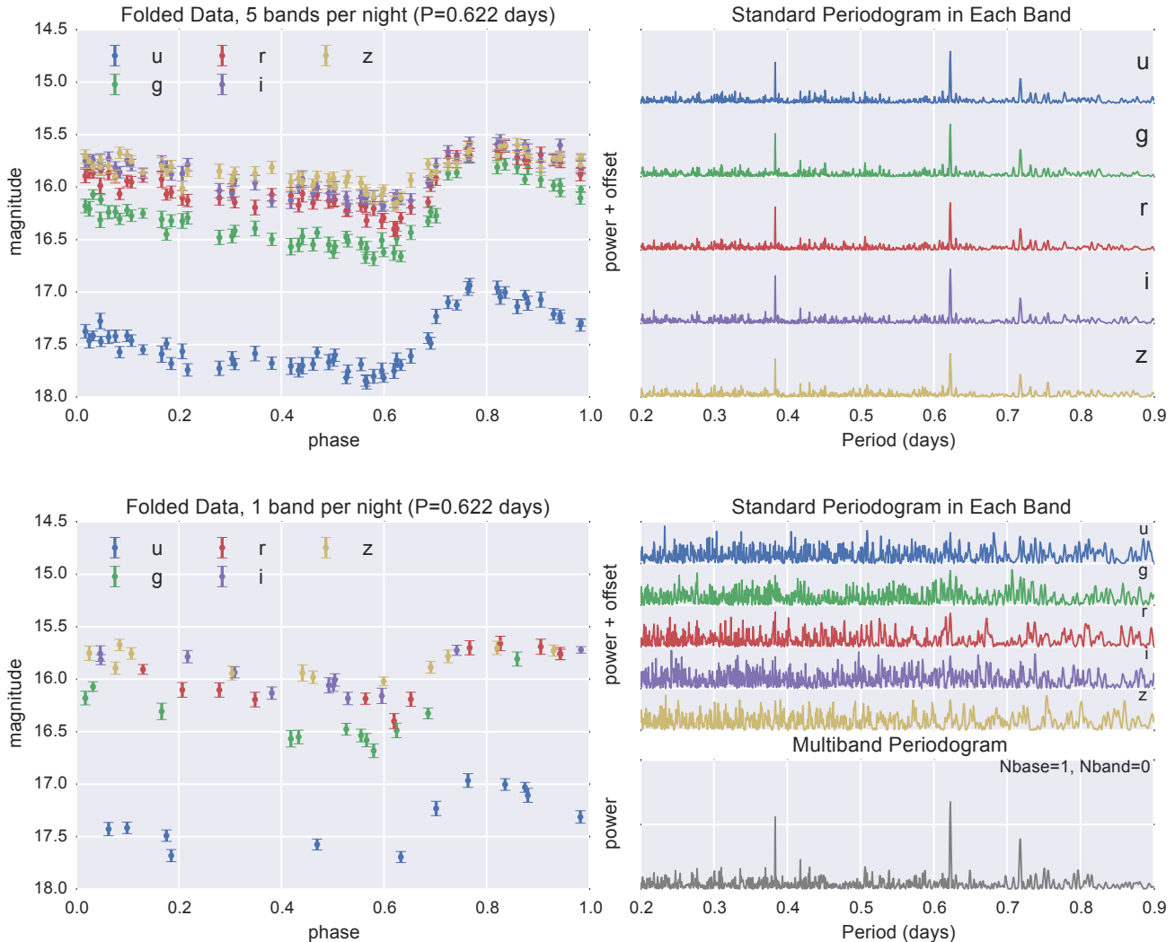
FIG. 5.— An illustration of the performance of the multiband periodogram. The upper panels show simulated ugriz observations of an RR Lyrae light curve in which all 5 bands are observed each night. With 60 observations in each band, a periodogram computed from any single band is sufficient to determine the true period of 0.622 days. The lower panels show the same data, except with only a single ugriz band observed each night (i.e. 12 observations per band). In this case, no single band has enough information to detect the period. The shared-phase multiband approach of Section 5 (lower-right panel) combines the information from all five bands, and results in a significant detection of the true period. This indicates that while methods based on the standard periodogram are suitable for densely-sampled multiband data, the multiband periodogram is superior for sparsely-sampled multiband observations.
