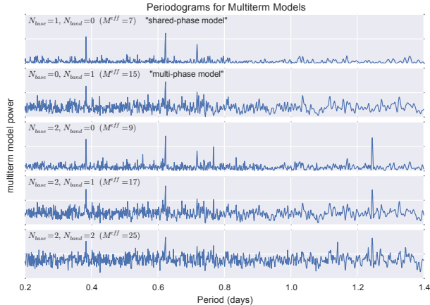
FIG. 6.— Comparison of the periodograms produced by various multiband models. The data is the same as that used in Figure 5. N_{base} gives the number of Fourier terms in the base model, and N_{band} gives the number of Fourier terms used to fit the residuals around this model within each band. The characteristics discussed with previous figures are also seen here: in particular, the level of “background noise” in the periodogram grows with the model complexity M ,
