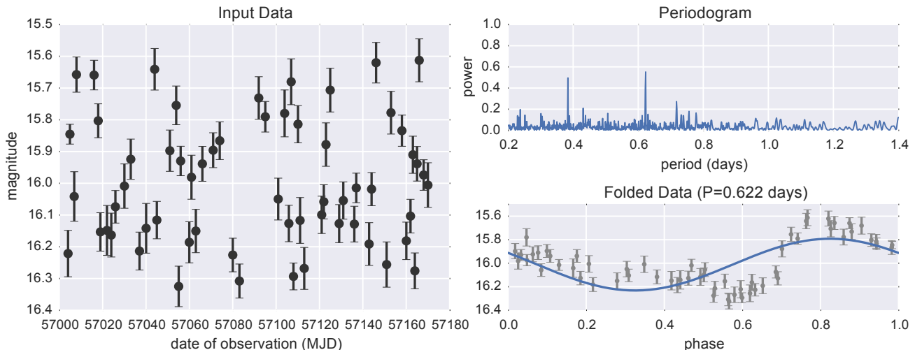
FIG. 1.— An illustration of the basic periodogram and its relationship to the single-term sinusoid model. The left panel shows the input data, while the right panels show the fit derived from the data. The upper-right panel shows the periodogram with a clear peak at the true period of 0.622 days, and the bottom-right panel shows the data as a function of the phase associated with this period. Note in the periodogram the presence of the typical aliasing effect, with power located at beat frequencies between the true period and the 1-day observing cadence (see Section 3.3 for further discussion).
