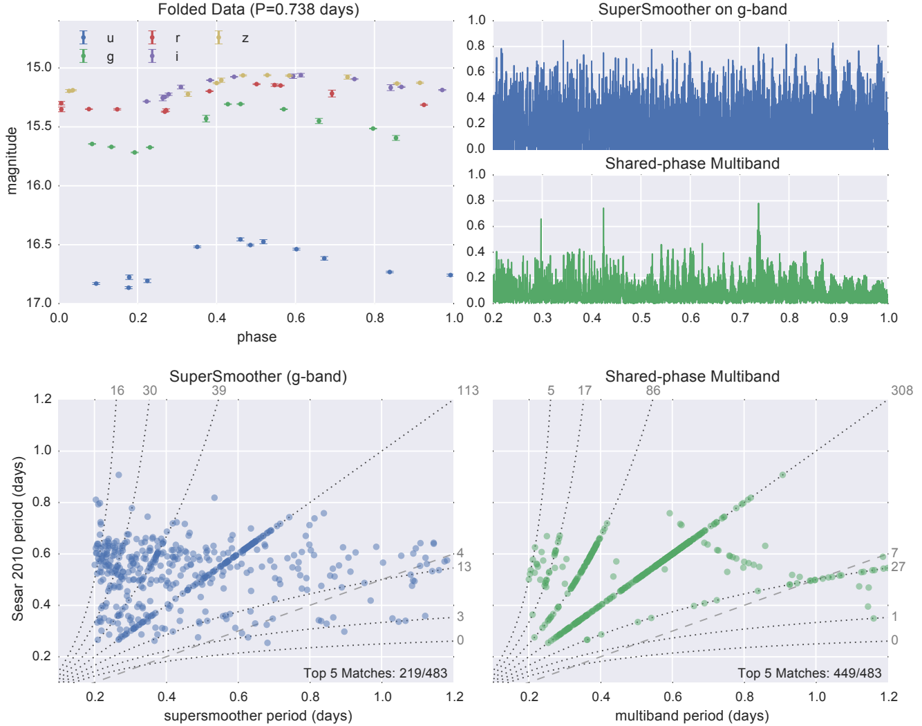
FIG. 8.— This figure repeats the experiment shown in Figure 7 (see caption there for description), but the data is artificially reduced to only a single-band observation on each evening, a situation reflective of the observing cadence of future large-scale surveys. In this case, the single-band SuperSmoother strategy used as a first pass in S10 fails: there is simply not enough data in each band to recover an accurate period estimate. The correct period is among the top 5 candidates in fewer than 50% of cases. The shared-phase multiband approach utilizes information from all five bands, and returns much more robust results: even with the greatly-reduced data, the true period is among the top 5 candidates in 93% of cases. This suggests that for sparsely-sampled multiband survey data (such as that expected from LSST) the multiband periodogram will produce superior results when compared to standard methods – see Figure 9.
