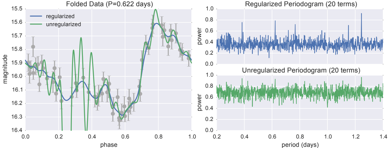
FIG. 4.— The effect of regularization on a high-order model. The data is the same as those in Figure 1. We fit a 20-term truncated Fourier model to the data, with and without a regularization term. Without regularization, the model oscillates widely to fit the noise in the data. The regularization term effectively damps the higher-order Fourier modes and removes this oscillating behavior, leading to a more robust model with stronger periodogram peaks.
