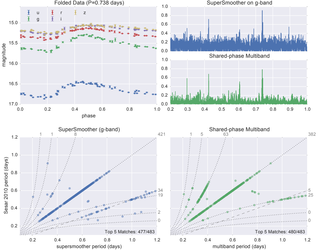
FIG. 7.— Comparison of the Multiband algorithm and single-band supersmoother algorithm on 483 well-sampled RR Lyrae light curves from Stripe 82. The upper panels show a representative lightcurve and periodogram fits, while the bottom panels compare the derived periods to the template-based periods reported in S10. Shown for reference are the beat aliases (dotted lines) and the first harmonic alias (dashed lines): numbers along the top and right edges of the panels indicate the number of points aligned with each trend. The single-band supersmoother model tends to err toward harmonic aliases, while the multiband model tends to err toward beat frequency aliases. Both methods find the correct period among the top 5 significant peaks around 99% of the time. This suggests that for densely-sampled multiband surveys, the multiband periodogram will match the results of standard methods (but see Figure 8).
