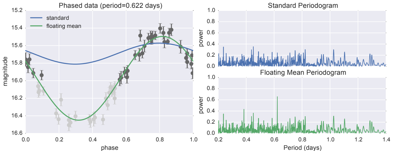
FIG. 2.— An illustration of the effect of the floating mean model for censored data. The data consist of 80 observations drawn from a sinusoidal model. To mimic a potentially damaging selection effect, all observations with magnitude fainter than 16 are removed (indicated by the light-gray points). The standard and floating-mean periodograms are computed from the remaining data; these fits are shown over the data in the left panel. Because of this biased observing pattern, the mean of the observed data is a biased estimator of the true mean. The standard fixed-mean model in this case fails to recover the true period of 0.622 days, while the floating mean model still finds the correct period.
