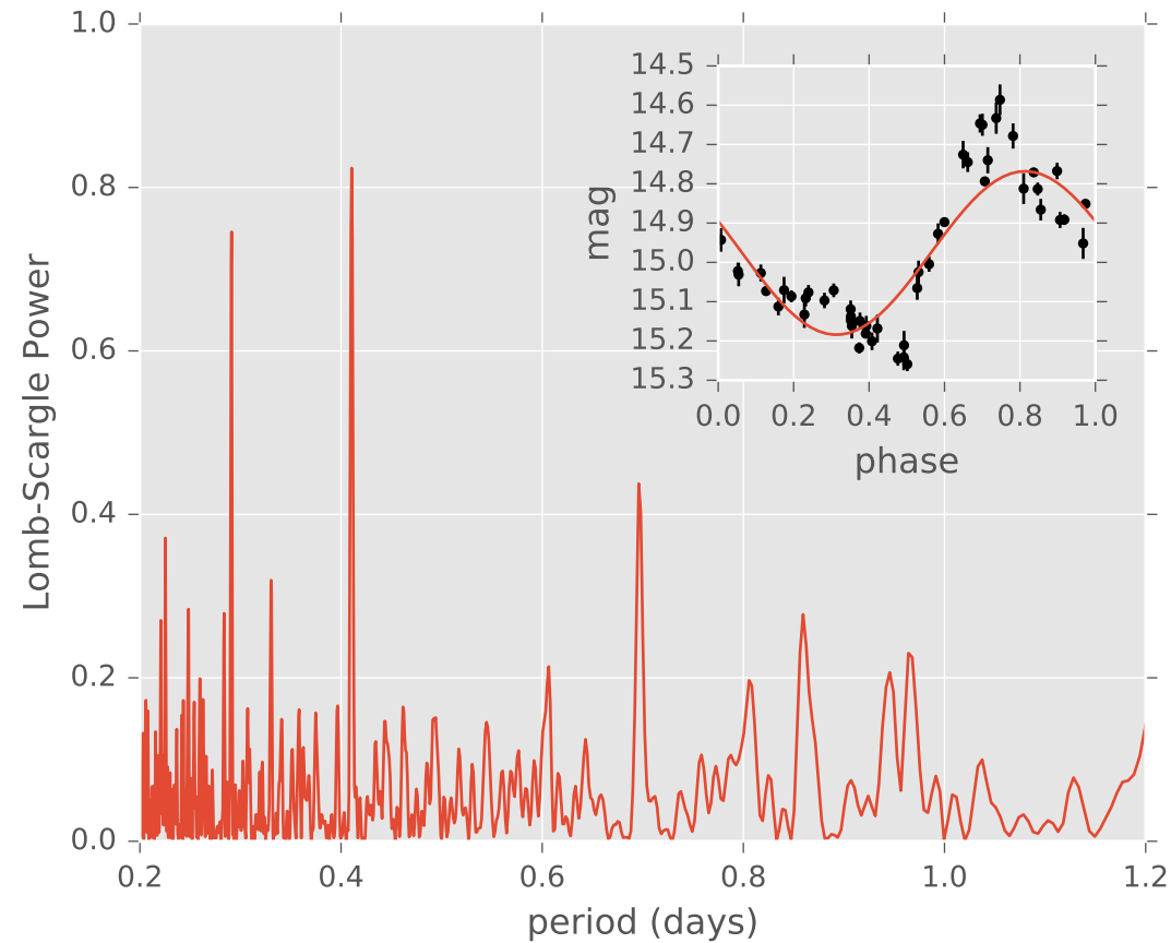
Lomb-Scargle Periodogram (period=0.41 days)
